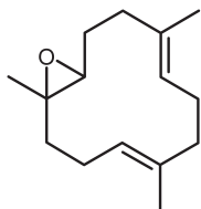
13-Oxabicyclo[10.1.0]trideca-4,8-diene, trimethyl-
